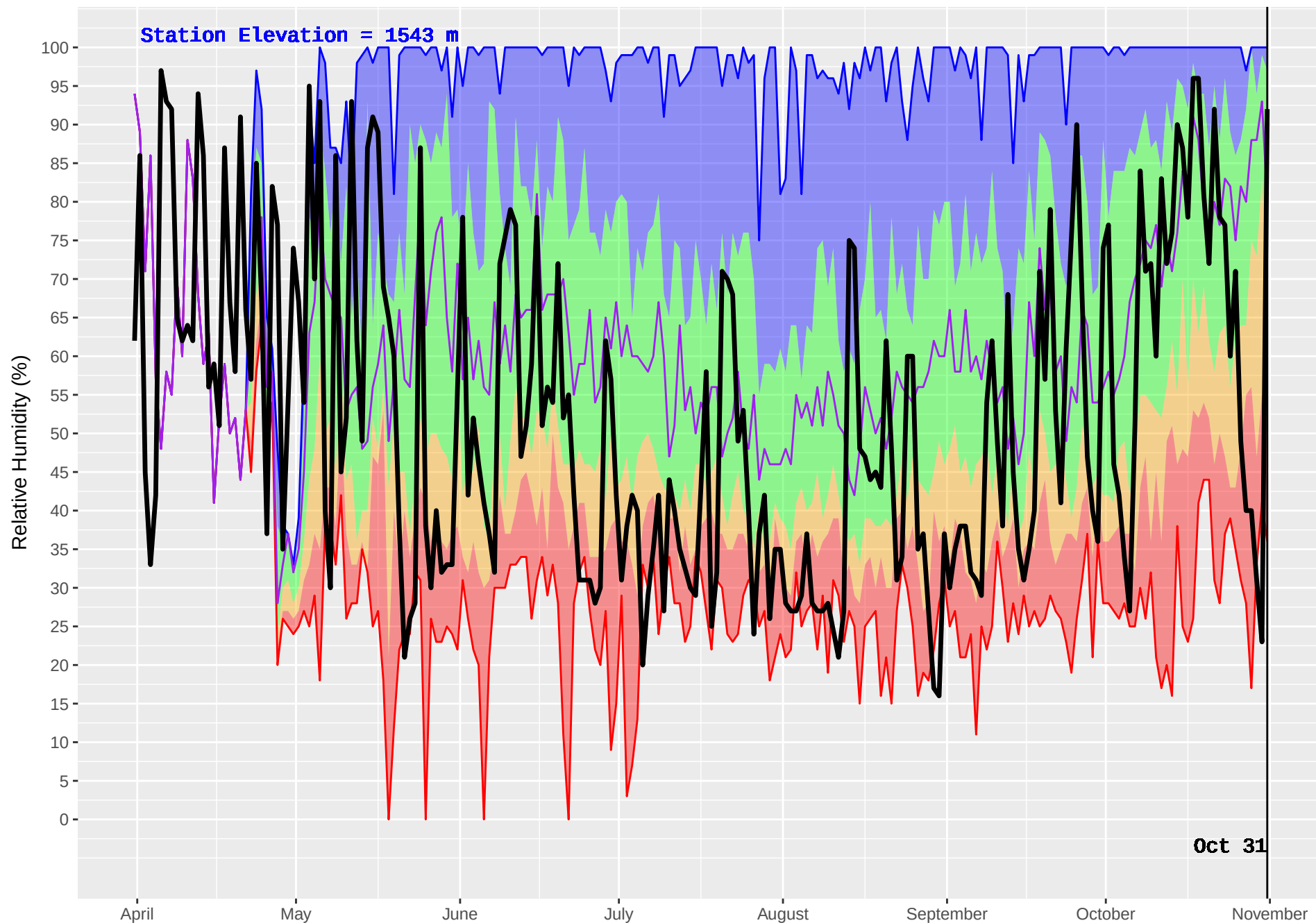
CAHILTY (253) : Historical (1987–2016) and Current (2017) Noon Relative Humidity
