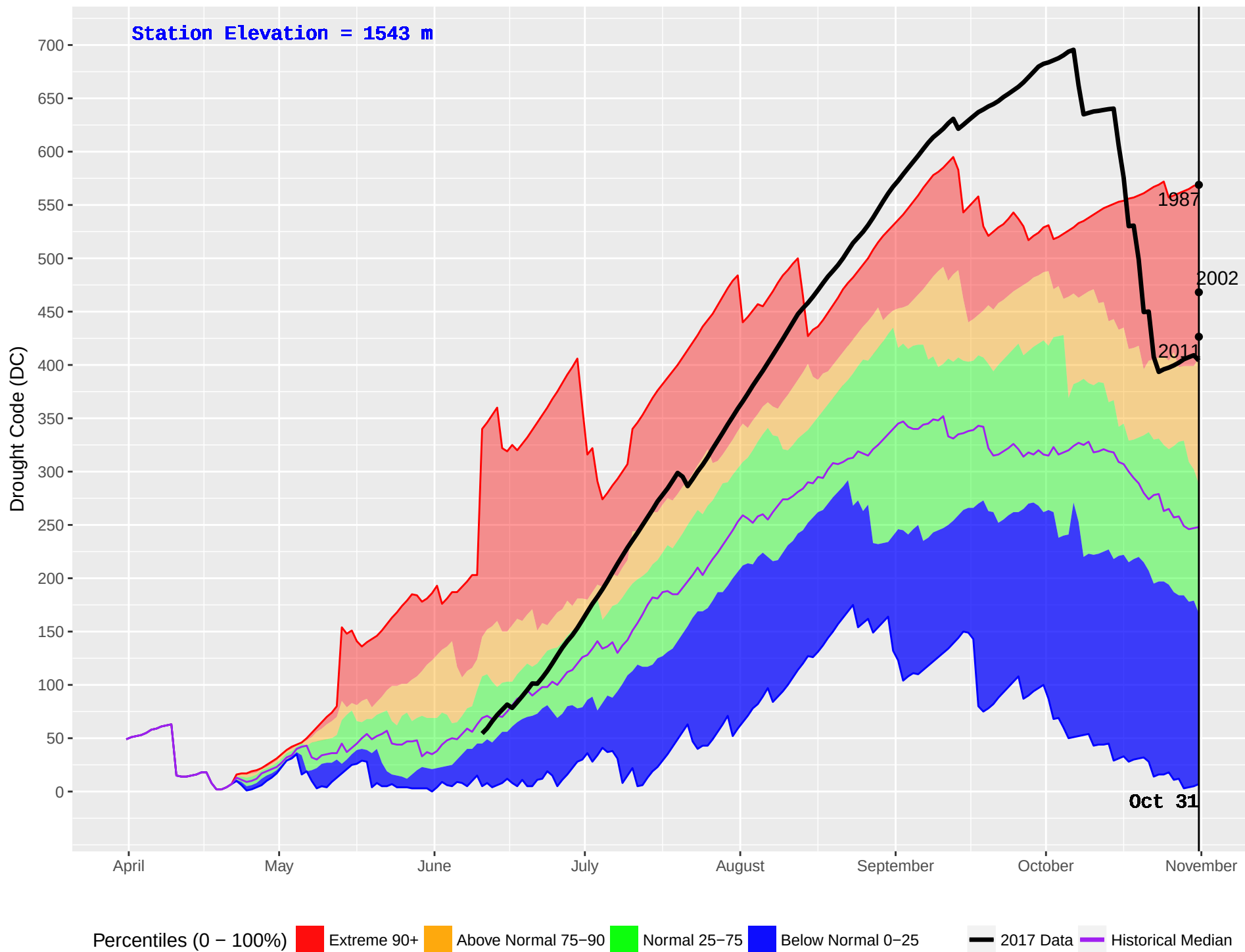
CAHILTY (253) : Historical (1987–2016) and Current (2017) Noon Drought Code (DC)
