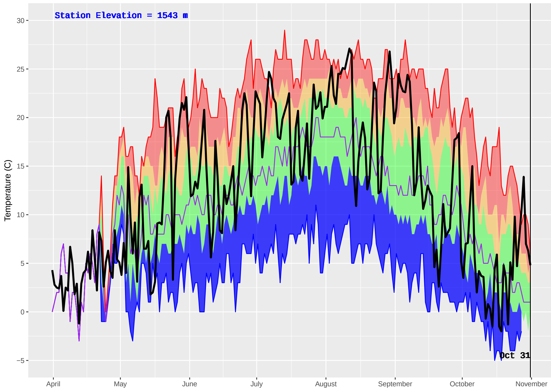
CAHILTY (253) : Historical (1987–2016) and Current (2017) Noon Temperature
