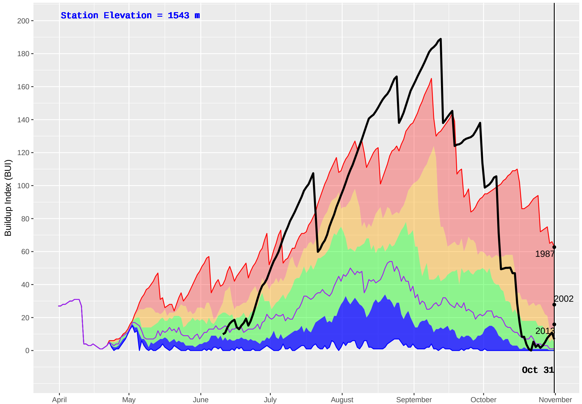
CAHILTY (253) : Historical (1987–2016) and Current (2017) Noon Buildup Index (BUI)
